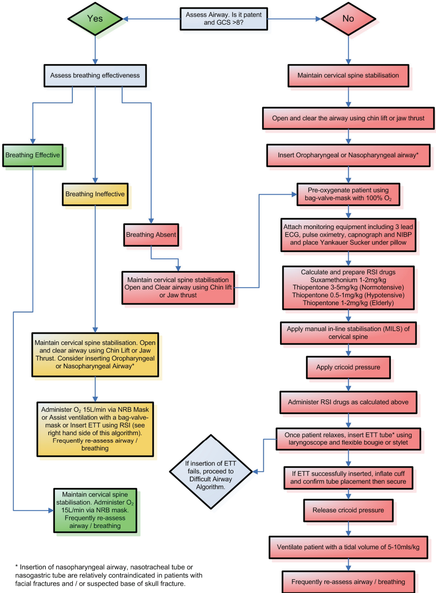
Algorithm 1:
